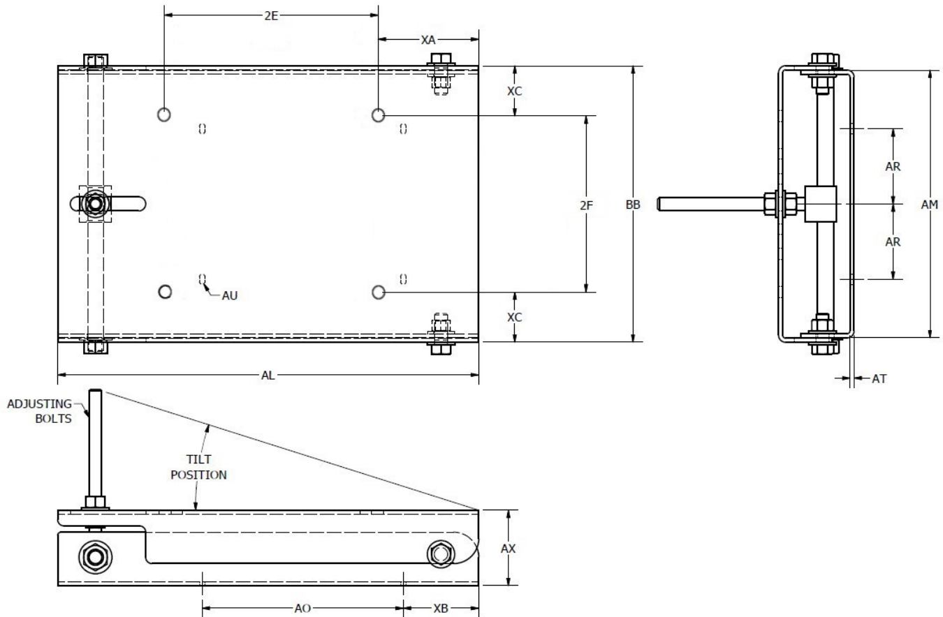
DIMENSION CHART FOR FIXED PIVOT BASES
