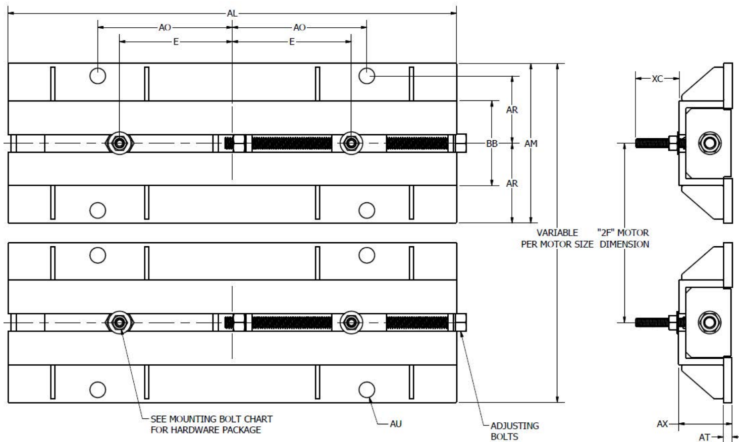
DIMENSION CHART FOR STRUCTURAL RAILS
