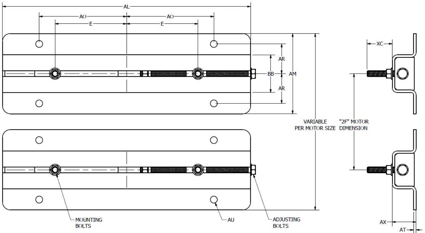
DIMENSION CHART FOR STANDARD RAILS STYLE 2
