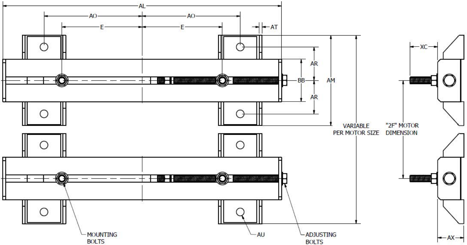
DIMENSION CHART FOR STANDARD RAILS STYLE 1
