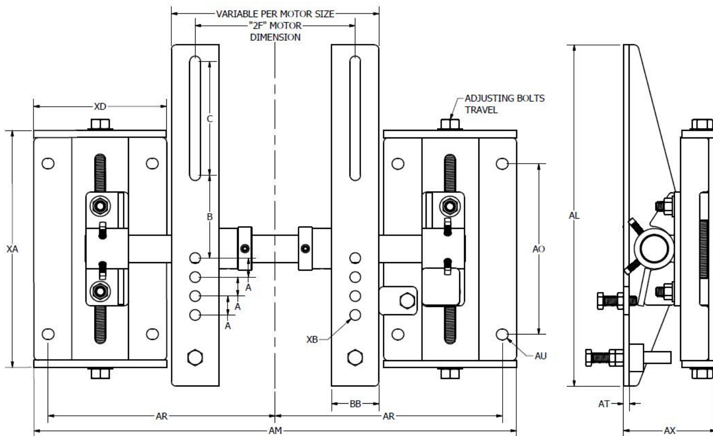
DIMENSION CHART FOR REACTIVE PIVOT BASES
