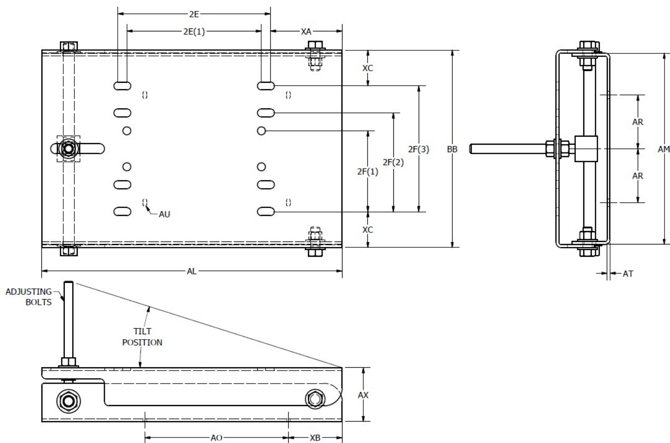
DIMENSION CHART FOR FIXED PIVOT BASES
