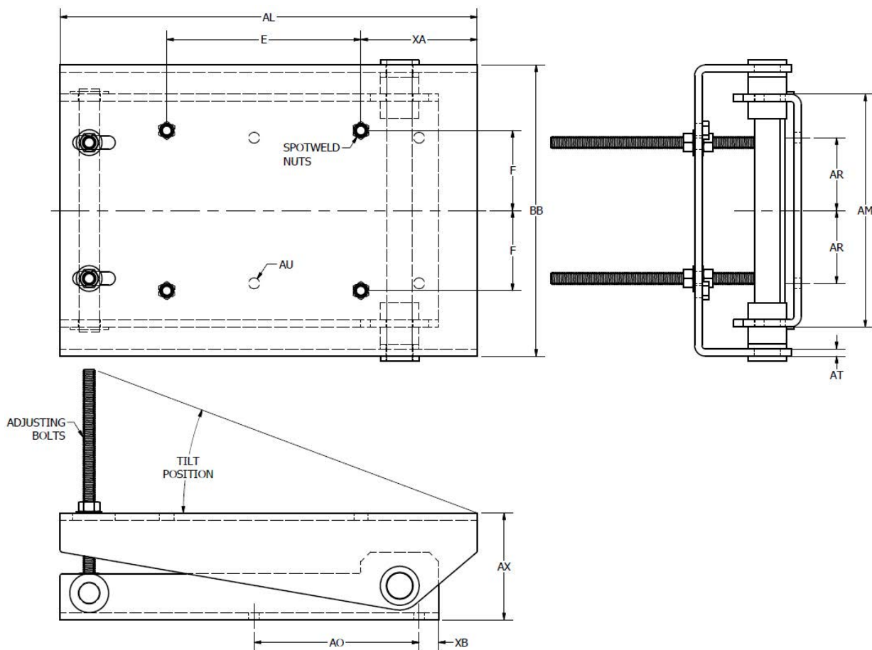
DIMENSION CHART FOR FIXED PIVOT BASES
