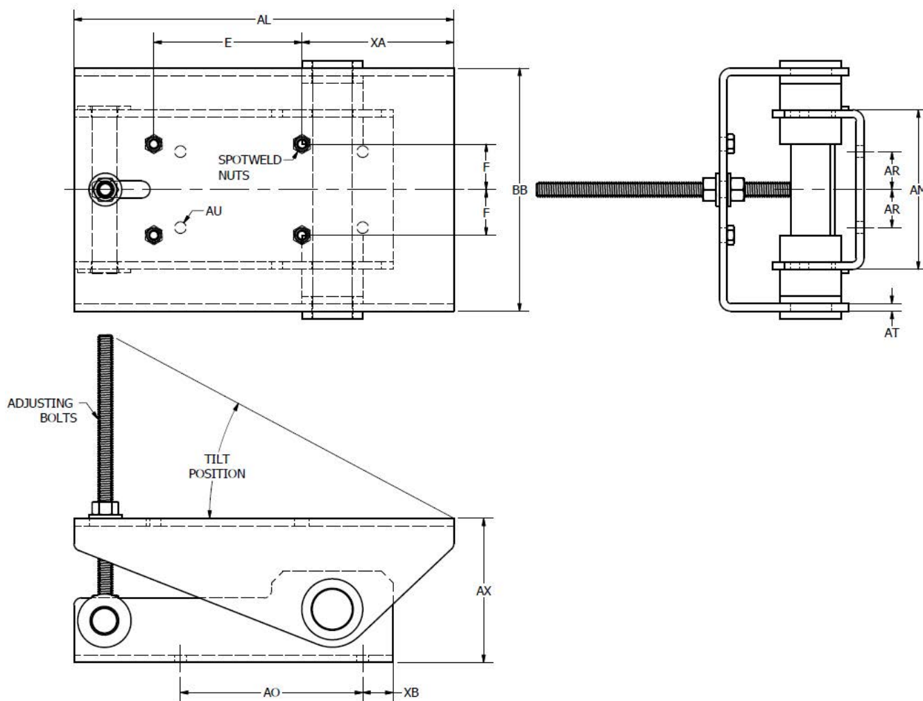
DIMENSION CHART FOR FIXED PIVOT BASES
