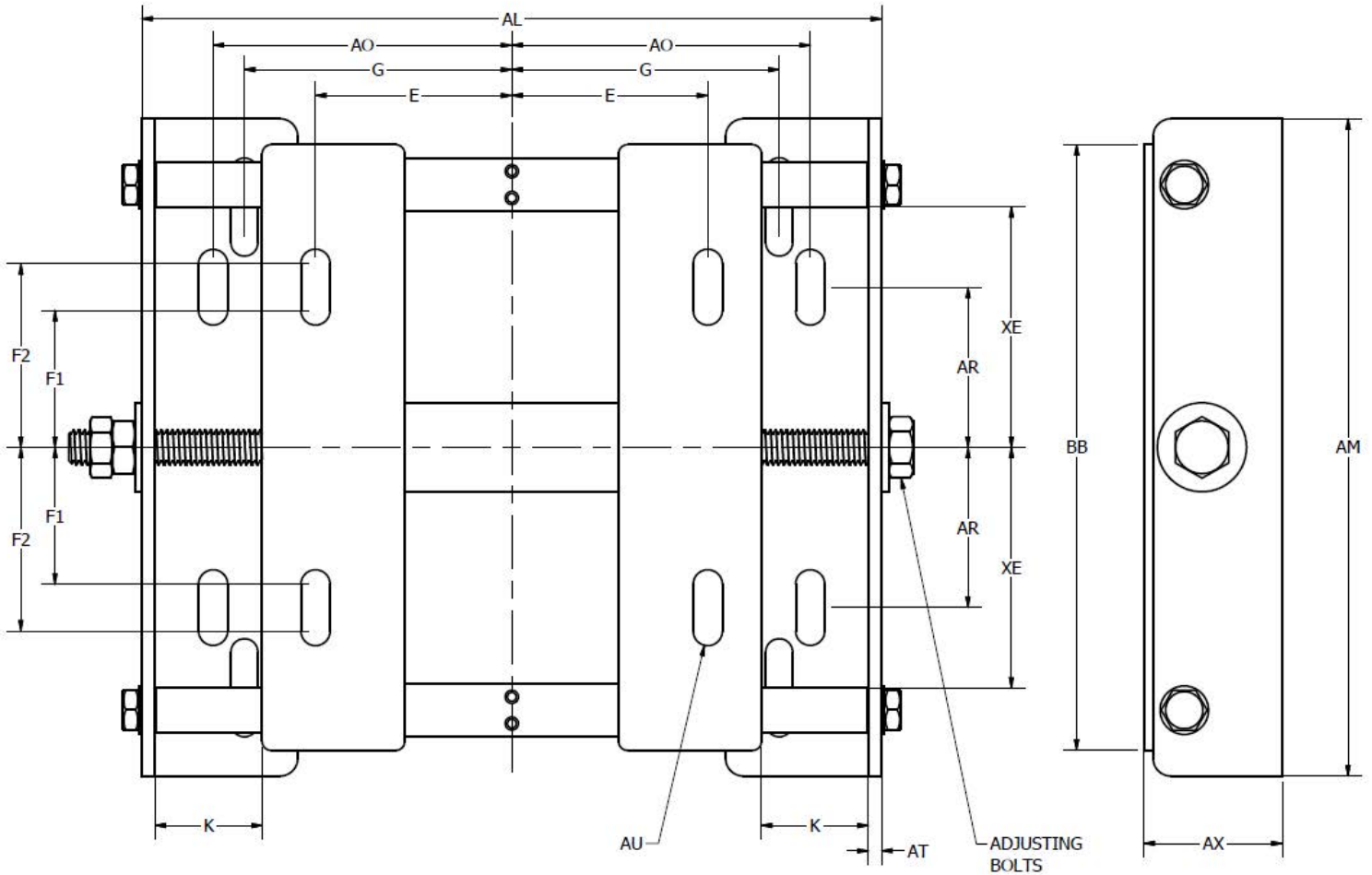
MOUNTING POSITION AND DIMENSIONS FOR 600 SERIES AUTOMATIC MOTOR BASES
