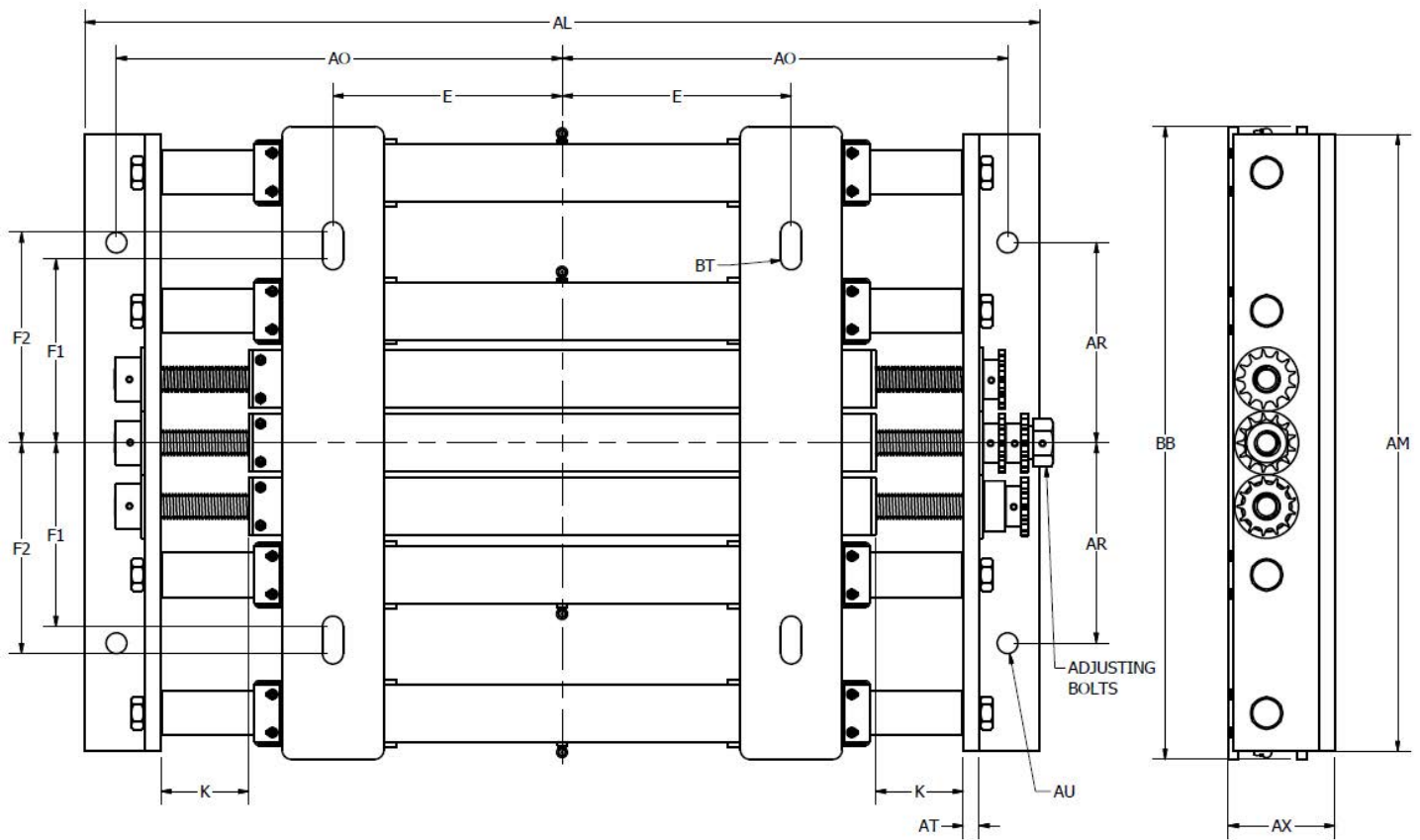
MOUNTING POSITION AND DIMENSIONS FOR DD1100 SERIES AUTOMATIC MOTOR BASES
